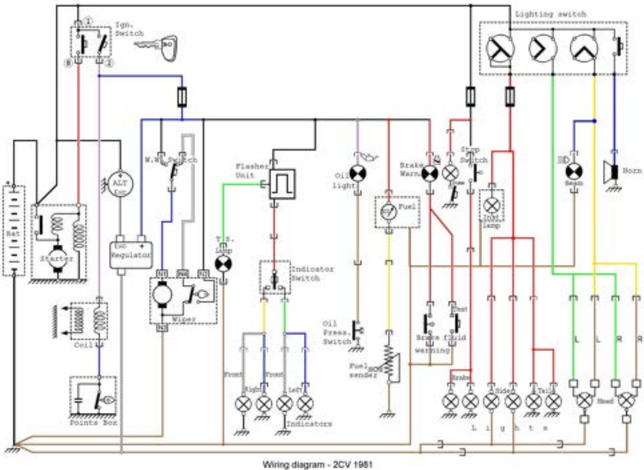
Fig. 4-5 2CV Electrical Wiring Diagram (Producer unknown)
